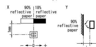
*2 Method of measuring position detection characteristic
