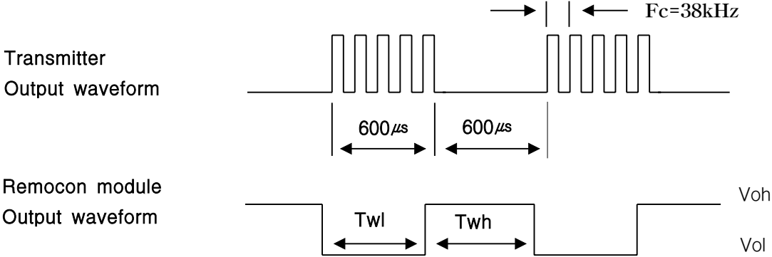
Fig 1. Output Waveform
