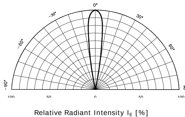
Fig. 5 Radiation Diagram
