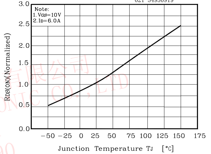
Fig.8 R_{DS(on)} - T_J
