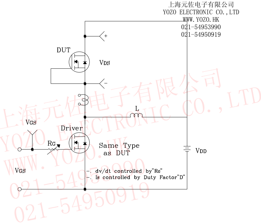
Fig. 13 Diode Reverse Recovery Time Test Circuit & Waveform
