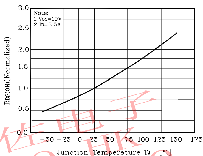
Fig.8 R_{DS(on)} - T_J
