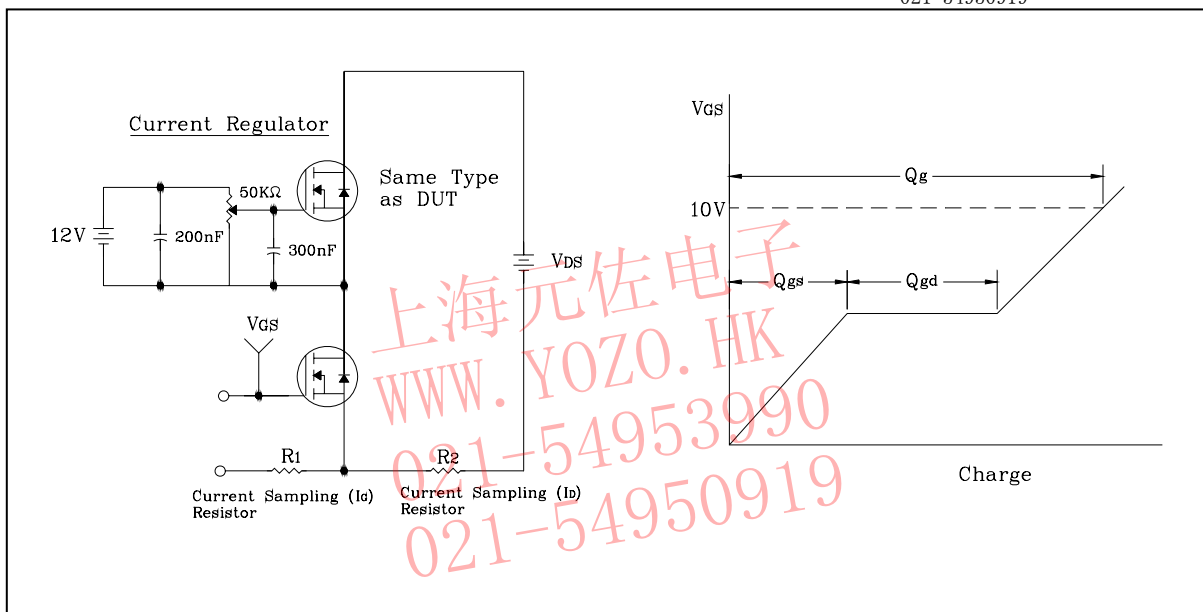
Fig. 11 Gate Charge Test Circuit &amp; Waveform
