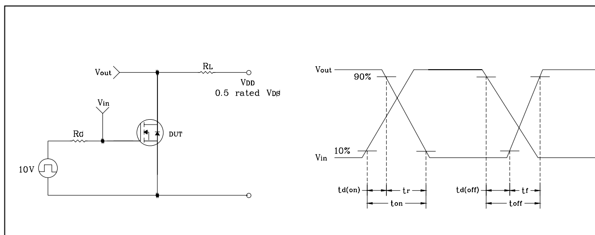
Fig. 12 Resistive Switching Test Circuit &amp; Waveform
